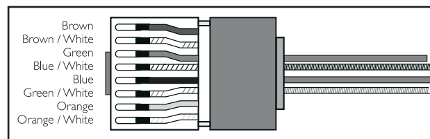
Figure 7-10: RJ45 Wiring and Pin Out Diagram
