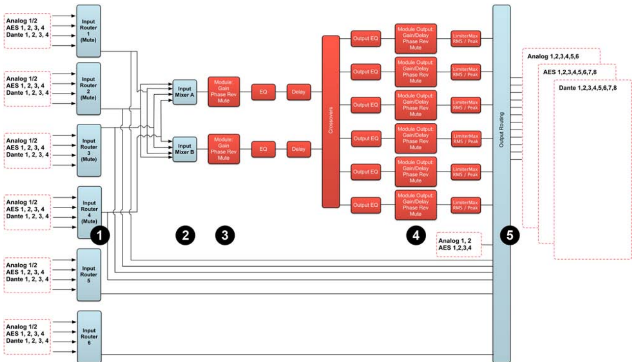
Figure 5-1: Signal Flow Diagram (LM 26)
