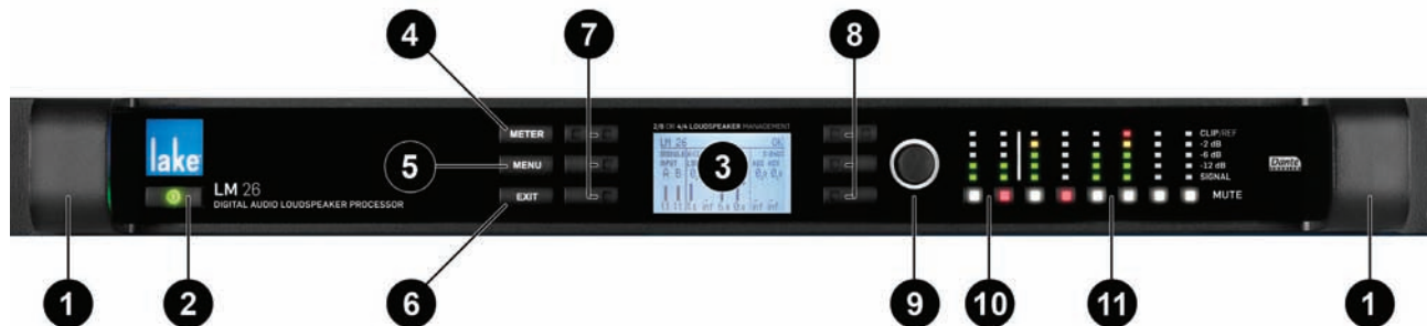
Figure 4-1: LM 26 Front Panel Overview
